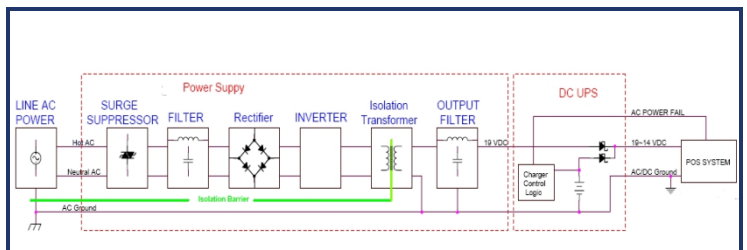
Block Diagram UPS – Power Supply AC Isolation Path
